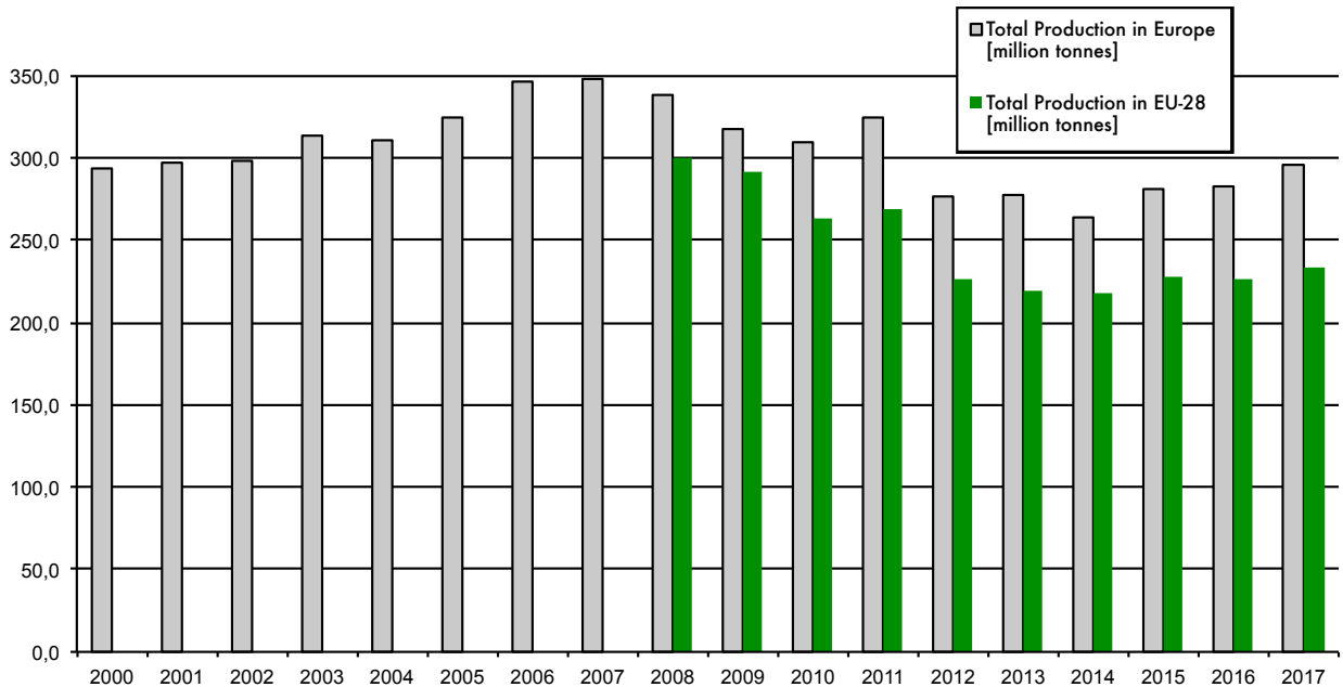
TOTAL PRODUCTION OF HOT AND WARM MIX ASPHALT IN EUROPE FROM 2000 TO 2017 (in million tonnes)
